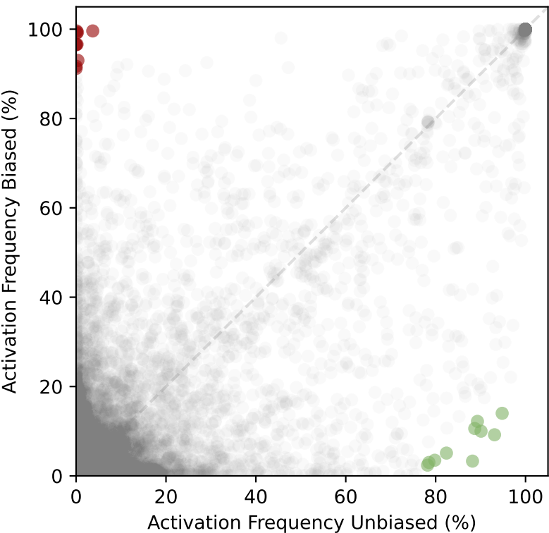
Activation Frequencies of SAE Latents: Pos_vs_neg
